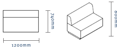
1200 Straight Lowback BOU002
