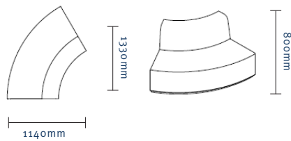
120D External Curve Lowback BOU009
