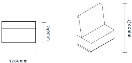
1200 Straight Highback BOU011
