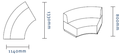
R500 External Lowback BOU008
